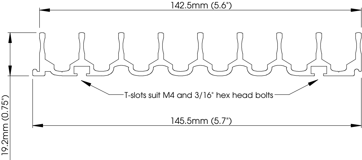
END VIEW - 2x MODULES
