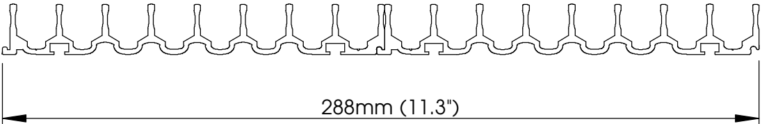
END VIEW - 2x MODULES
